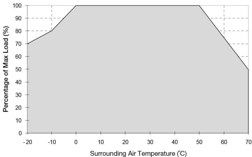
Fig. 1 De-rating for Vertical and Horizontal Mounting Orientation -20°C to -10°C de-rate power by 1% / °C, -10°C to 0°C de-rate power by 2% / °C, > 50°C de-rate power by 2.5% / °C
