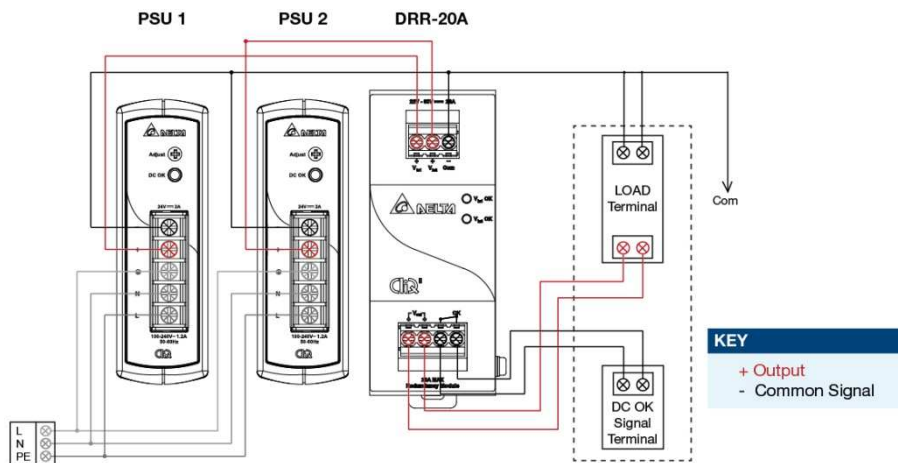
Fig. 2 Redundancy / Parallel Operation Connection Diagram
