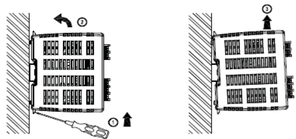
Fig. 2.2 Dismounting
