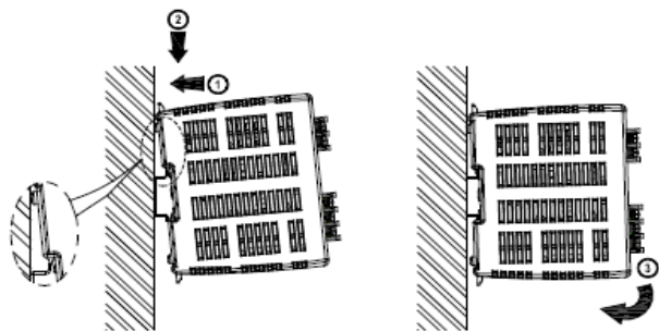
Fig. 2.1 Mounting
