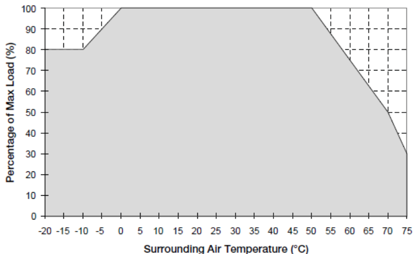
Fig. 1.1 De-rating for Vertical Mounting Orientation
