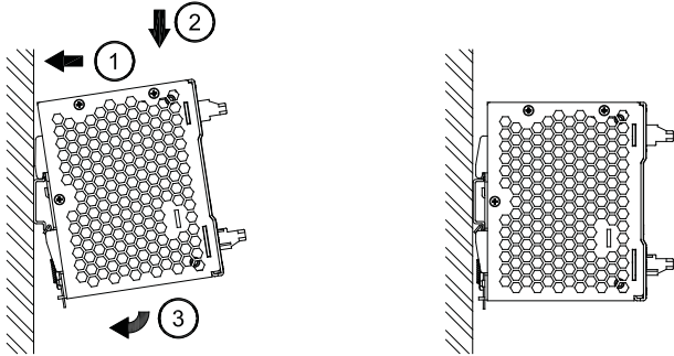
Fig. 3.1 Mounting
