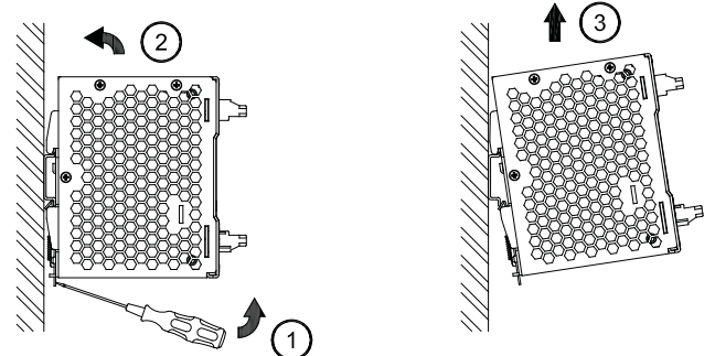
Fig. 3.2 Dismounting
