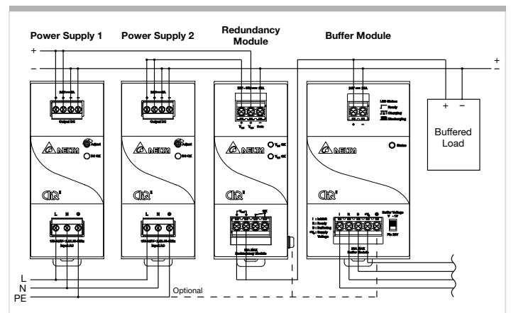
Fig. 4.6 Connection Diagram with Redundant Operation
