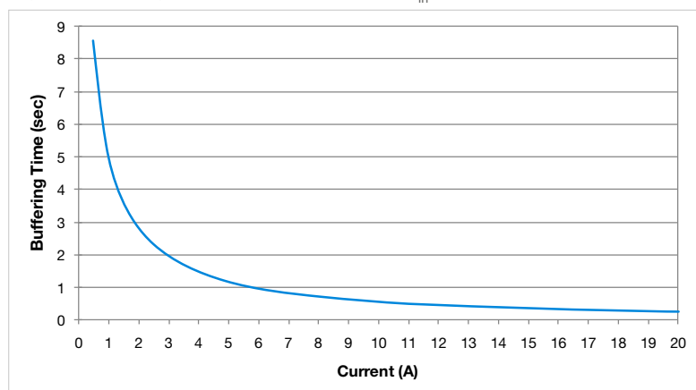
Fig. 1 Buffering Time (Typical Values at " V_{in}-1V " Mode)
