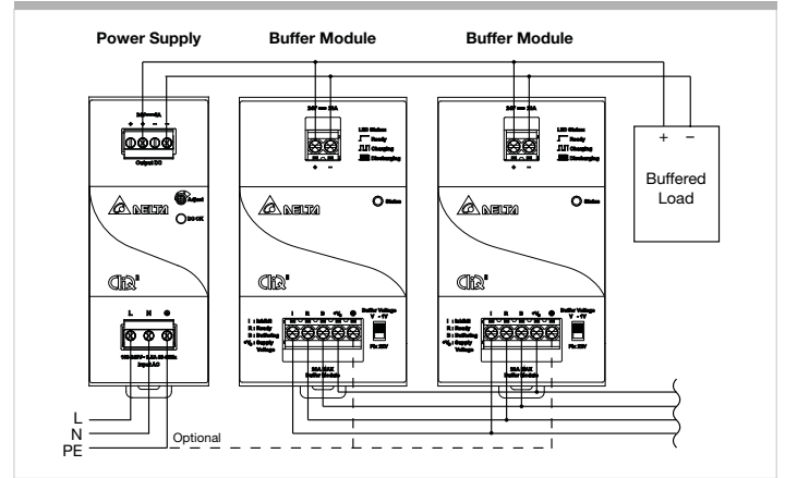
Fig. 4.2 Paralleling of Buffer Units
