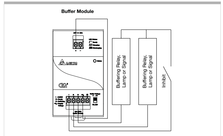
Fig. 4.4 General Signals Wiring
