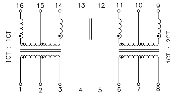
SCHEMATIC
