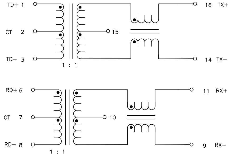
SCHEMATIC
