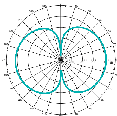
2.45GHz 1.6233dBi
