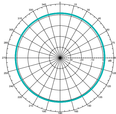
2.4GHz 1.55524dBi
