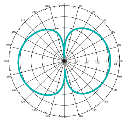
2.5GHz 1.59034dBi
