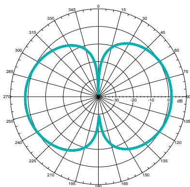
2.4GHz 1.61476dBi
