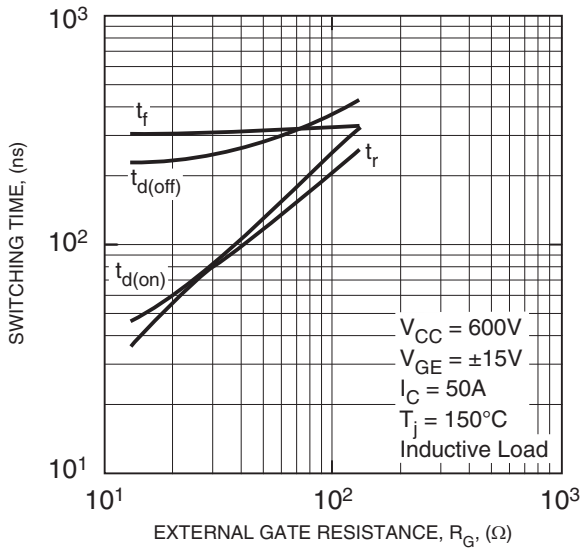
SWITCHING TIME VS. GATE RESISTANCE (BRAKE - TYPICAL)
