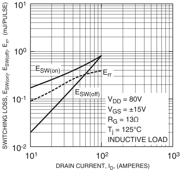
SWITCHING LOSS VS. DRAIN CURRENT (TYPICAL)
