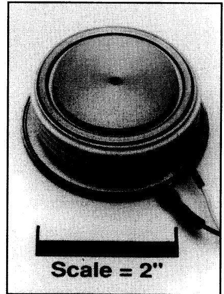
C451 Phase Control SCR 1500 Amperes Average, 2400 Volts
