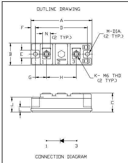
QRS0620T30 Fast Recovery Diode Module
