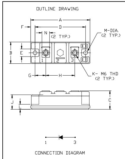
QRS1260T30 Fast Recovery Diode Module
