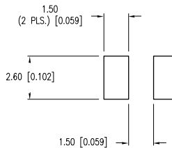
RECOMMENDED SOLDER PAD LAYOUT
