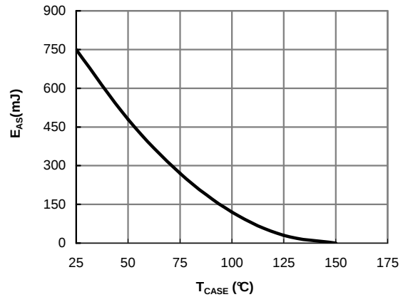
Figure 14: Avalanche energy
