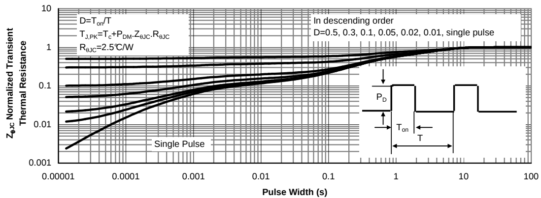
Figure 13: Normalized Maximum Transient Thermal Impedance for AOTF12N65 (Note F)
