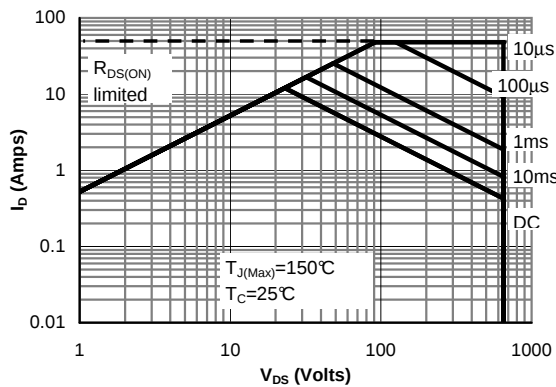
Figure 9: Maximum Forward Biased Safe Operating Area for AOT12N65 (Note F)
