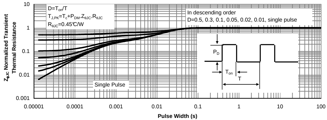
Figure 12: Normalized Maximum Transient Thermal Impedance for AOT12N65 (Note F)
