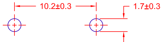
PC-BOARD PATTERN
