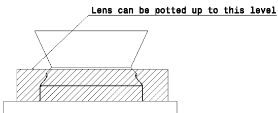
Potting with appropriate resin
