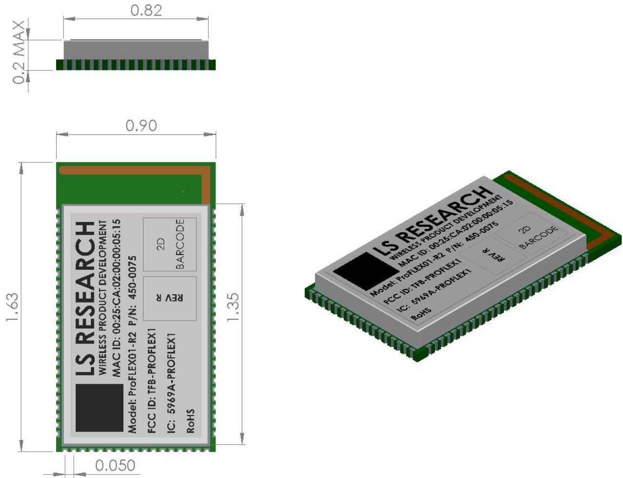
Figure 8 Basic dimensions
