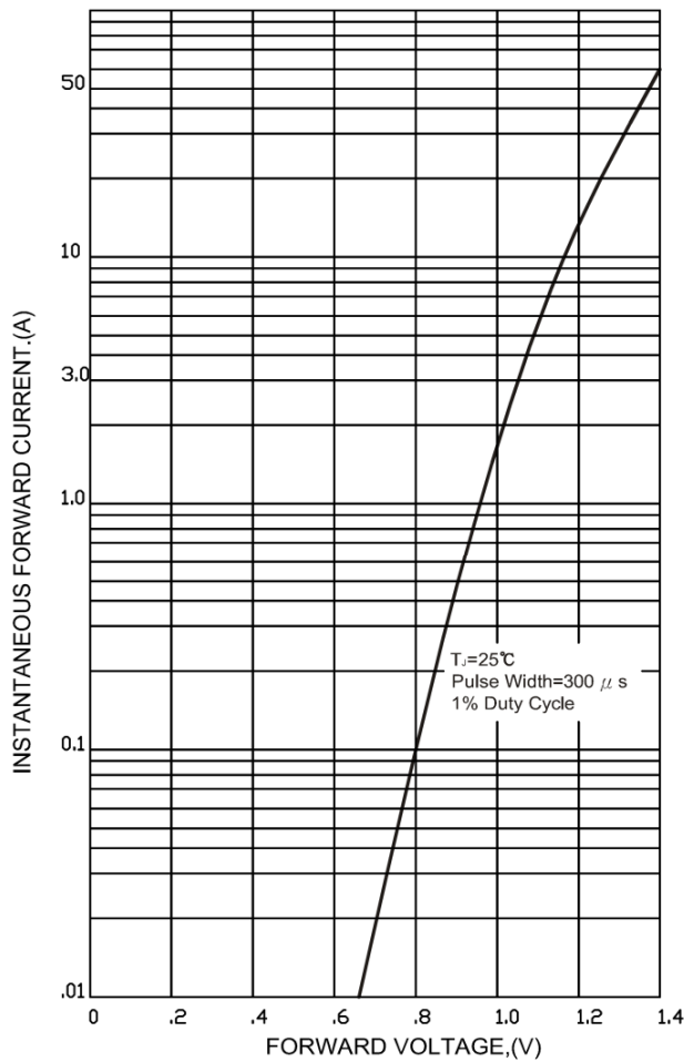
FIG.3-TYPICAL FORWARD CHARACTERISTICS
