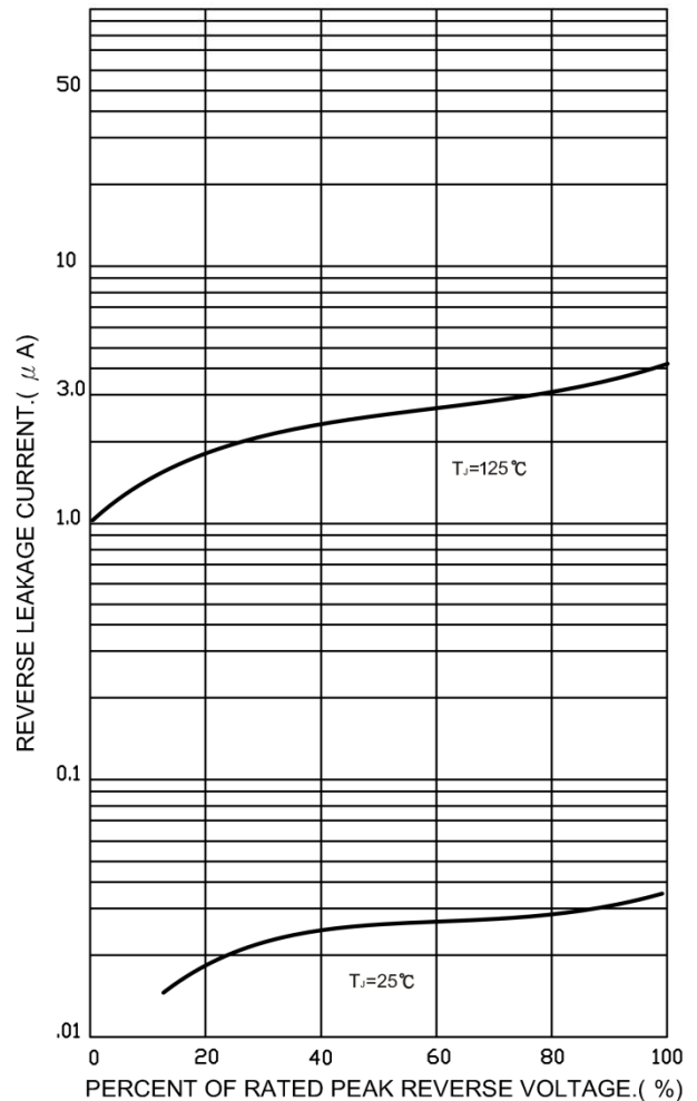
FIG.4-TYPICAL REVERSE CHARACTERISTICS
