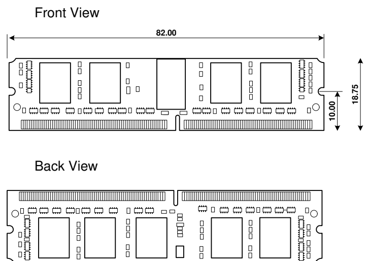
Figure: mechanical dimensions 1
