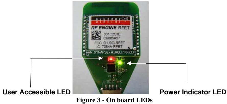
Figure 3 - On board LEDs
