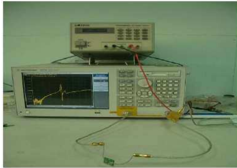
Figure 4. Network Analyzer
