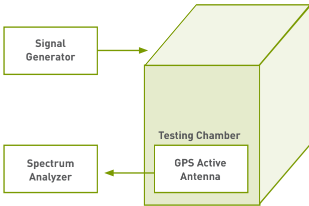
Testing Chamber
