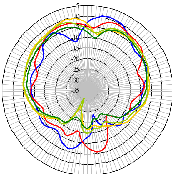
TG.09 90° in free space
