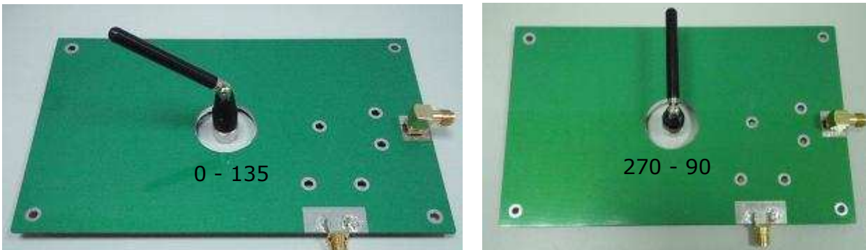
Different antenna mounting is marked as ( \varnothing angle-- \theta angle ), photos are two example of the position marking.
