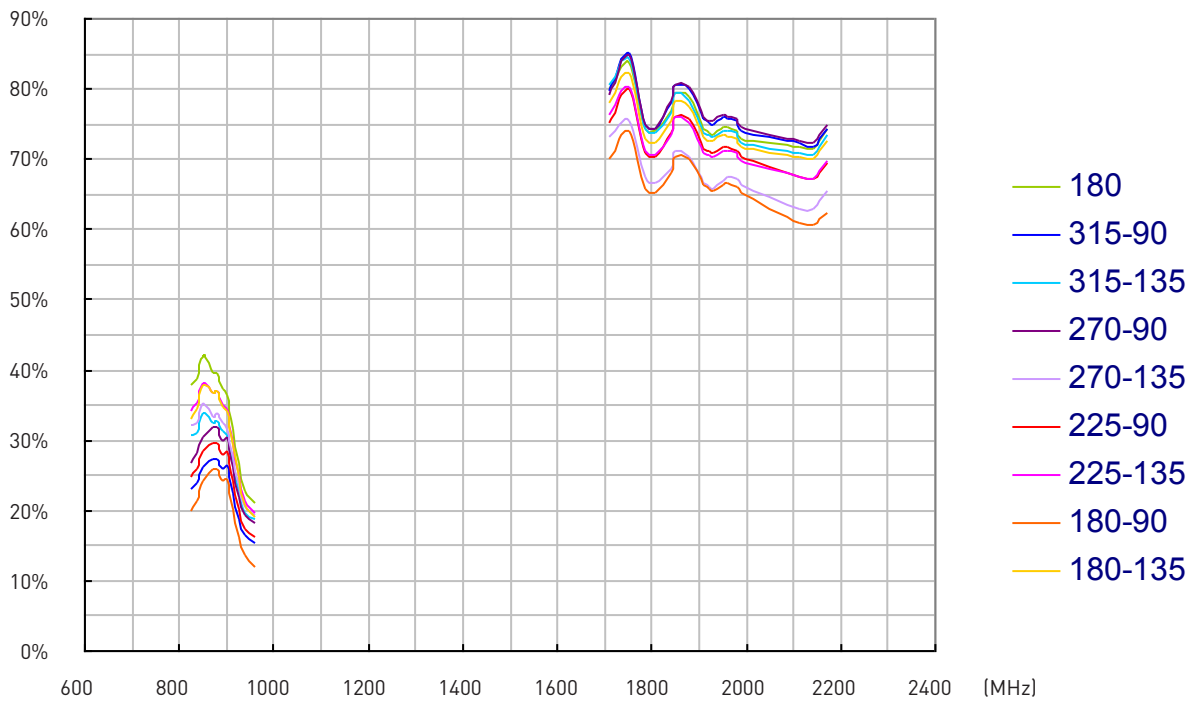
TG.09 mounted at the edge of PCB (upright position)
