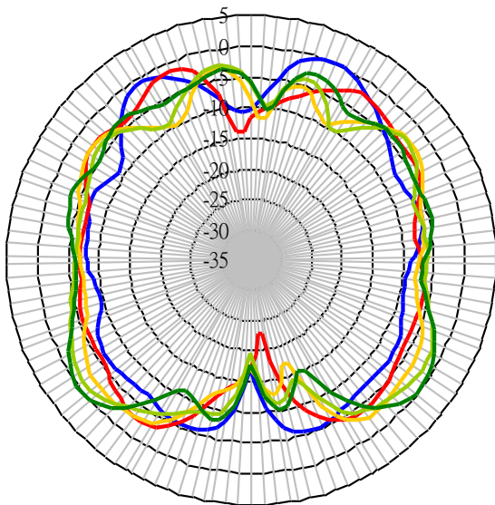
TG.09 90° mounted on metal plane (0-90)
