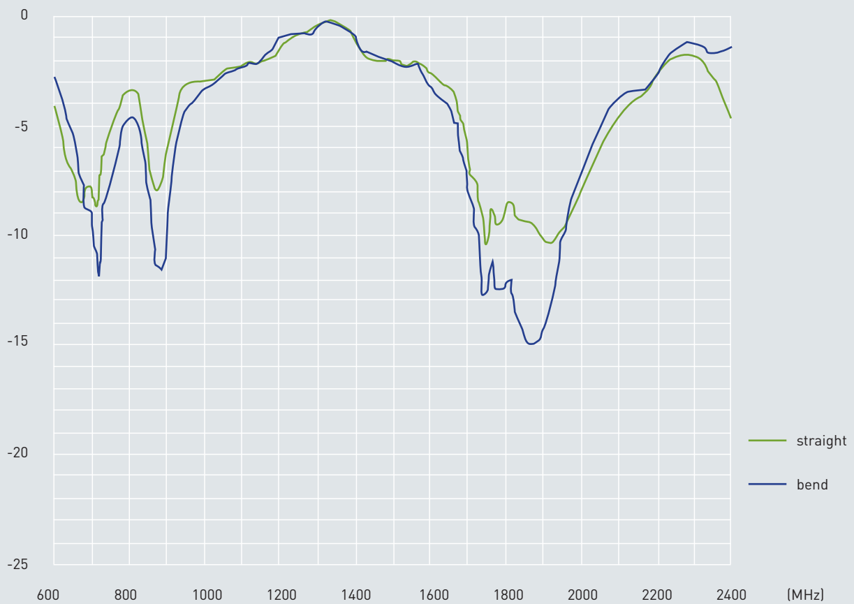
TG.09 tested with Agilent 8753ES
