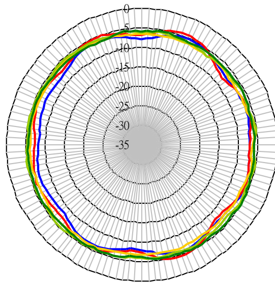
TG.09 90° mounted on metal plane (0-90)
