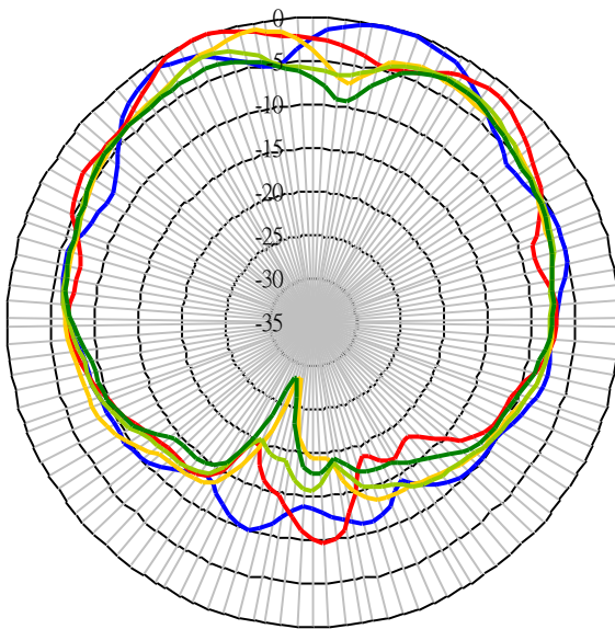
TG.09 90° in free space
