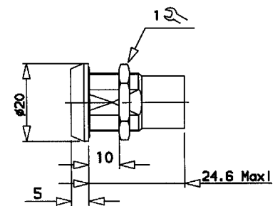
HM : Sealed Rear Mount Receptacle
