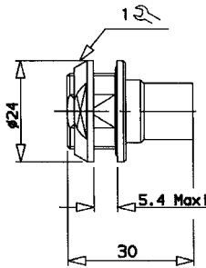
HG : Sealed Front Mount Receptacle
