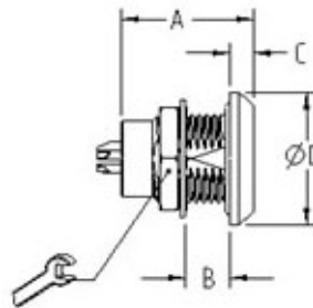
FE : Sealed Straight Plug with cable clamping
