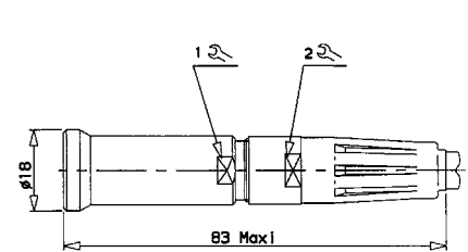
PE : Sealed In Line Receptacle
