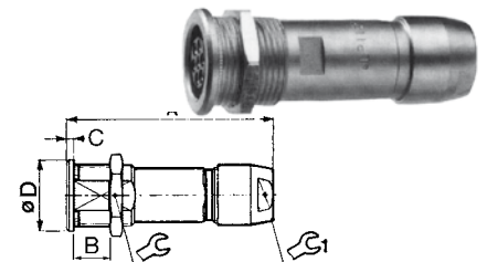
SR : Front Mount Cable Receptacle
