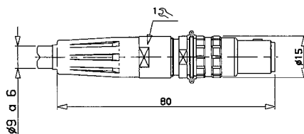
FE : Sealed Straight Plug with cable clamping
