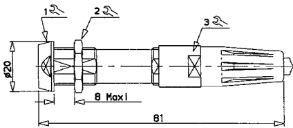
SE : Sealed Sealed Panel Mount Cable Receptacle
