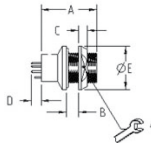
HM : Sealed Rear Mount Receptacle
