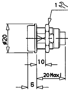
SE : Sealed Sealed Panel Mount Cable Receptacle
