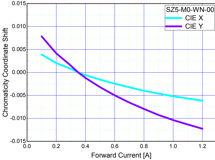
Forward Current vs. Chromaticity Coordinate, Ta=25°C
