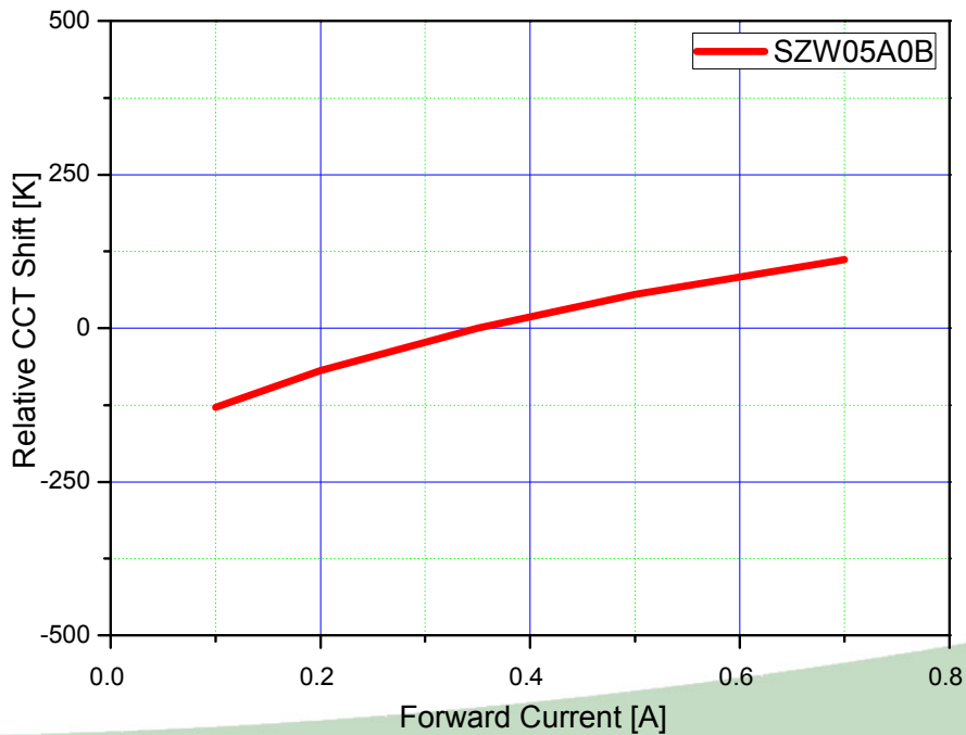
Forward Current vs. CCT, Ta=25℃
