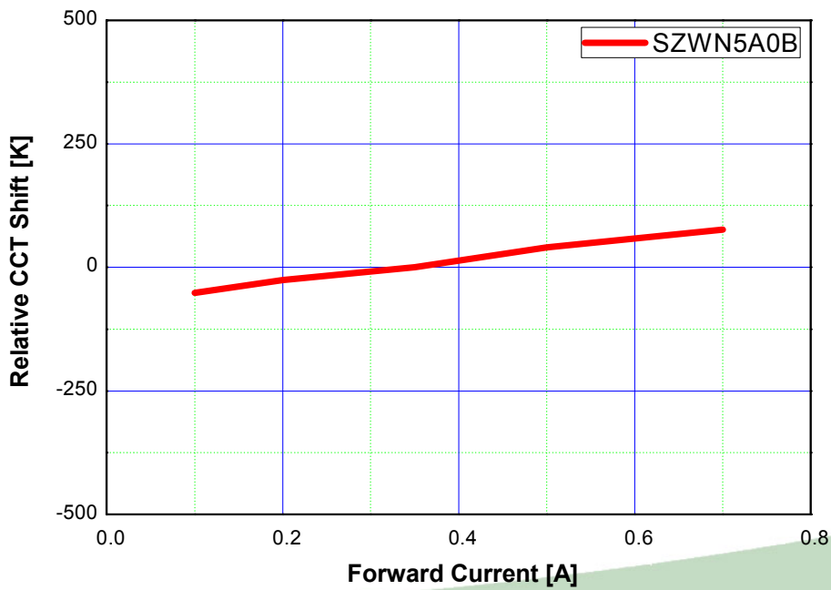
Forward Current vs. CCT, Ta=25℃
