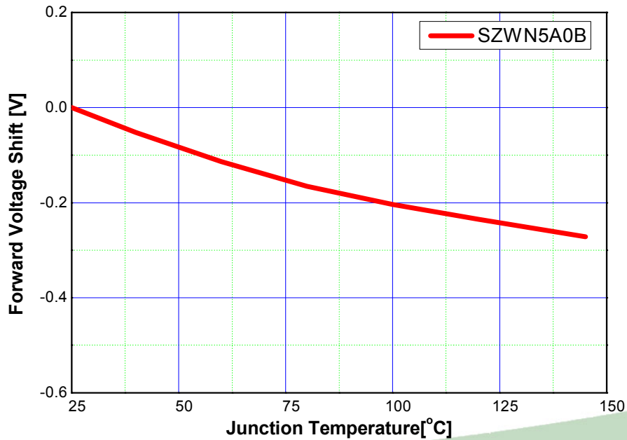
Junction Temperature vs. Forward Voltage at IF=350mA
