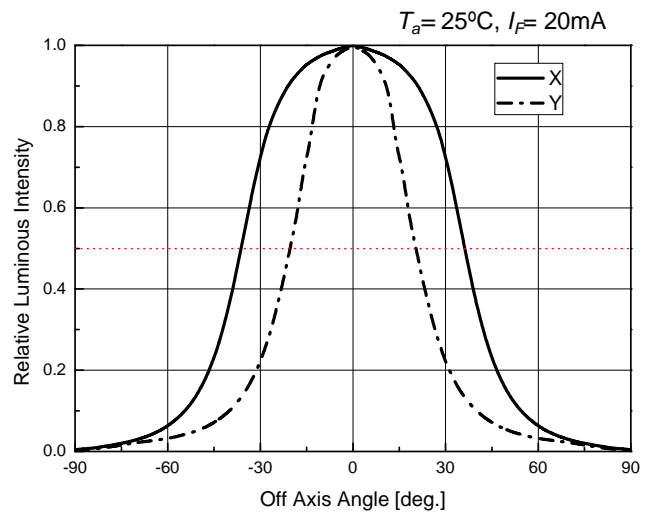
Directivity
