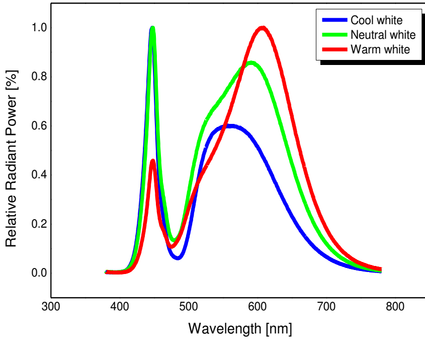
Fig 1. Color Spectrum, Ta = 25°C, IF = 700mA, RH30%
