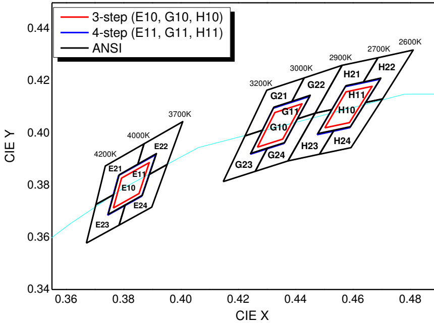
CIE Chromaticity Diagram (Warm white), Ta=25°C, IF=700mA
