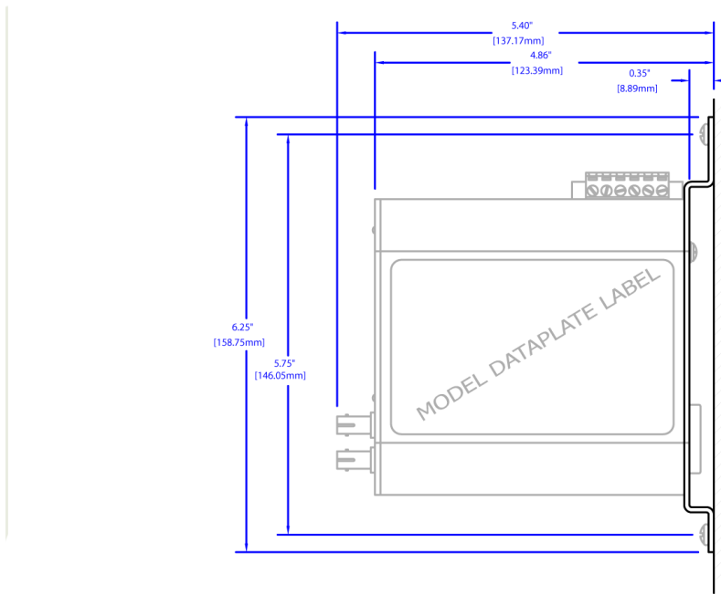
OPTIONAL COMPACT PANEL MOUNT ASSY. ( P/N: CPMA-1 )
