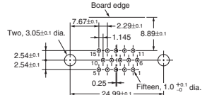
Mounting holes (t = 1.6 mm, bottom view)
