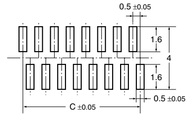
Printed Circuit Board Matching Dimensions (Top View)
