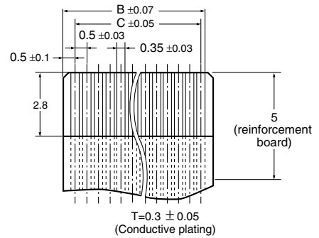
Applicable FPC Dimensions
