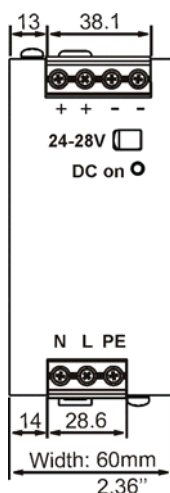
Fig. 22-1 Front view
