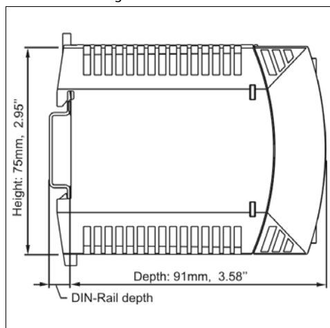
Fig. 20-2 Side view
