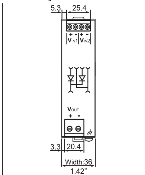
Fig. 16-1 Front view
