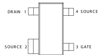
SOT-343 (SC-70) PACKAGE
