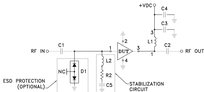
Fig 2b. Evaluation board unconditionally stable (see note AN-60-064)
