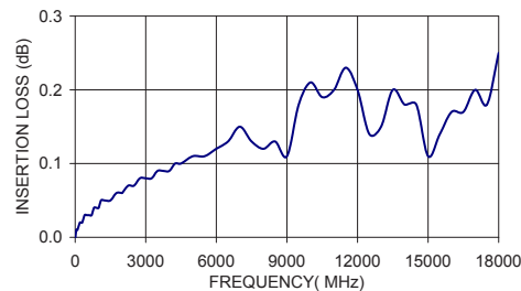
141-4SM+ INSERTION LOSS
