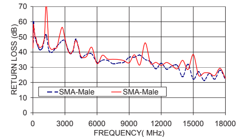
141-4SM+ RETURN LOSS
