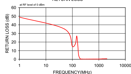
SALF-146 RETURN LOSS
