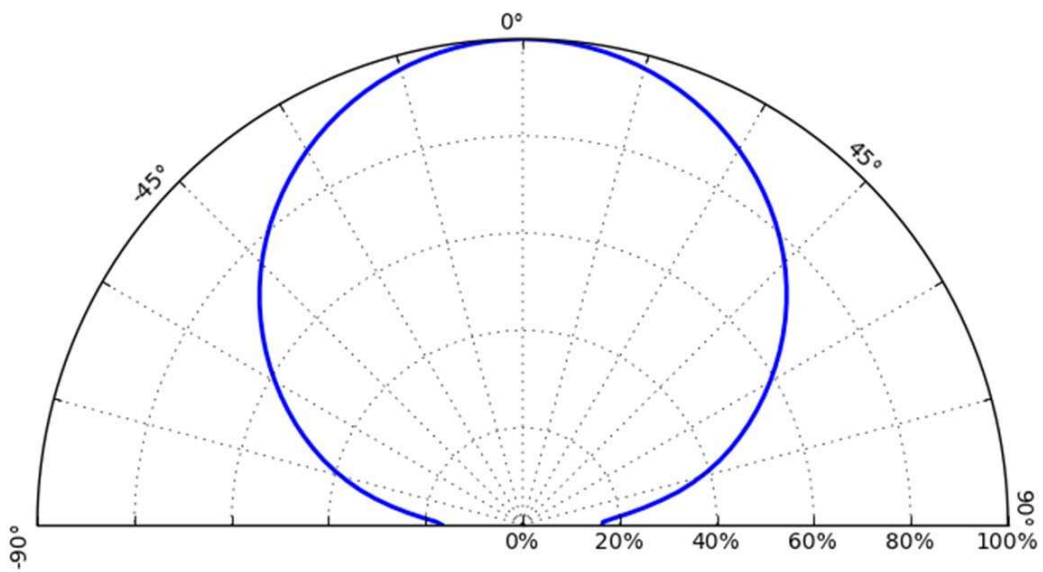
Figure 10. Typical representative polar radiation pattern for LIQ0-xyy00000zzz0.
