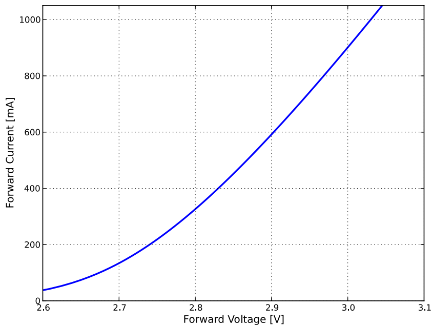
Figure 8. Typical forward current vs. forward volatage, LIQ0-xyy00000zzz0.
