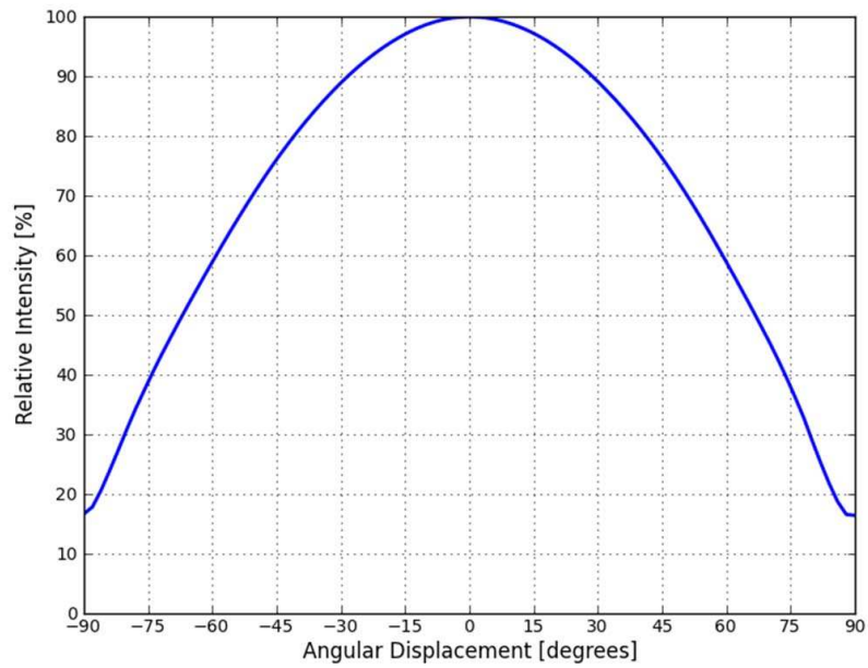
Figure 9. Typical representative spatial radiation pattern for LIQ0-xyy00000zzz0.
