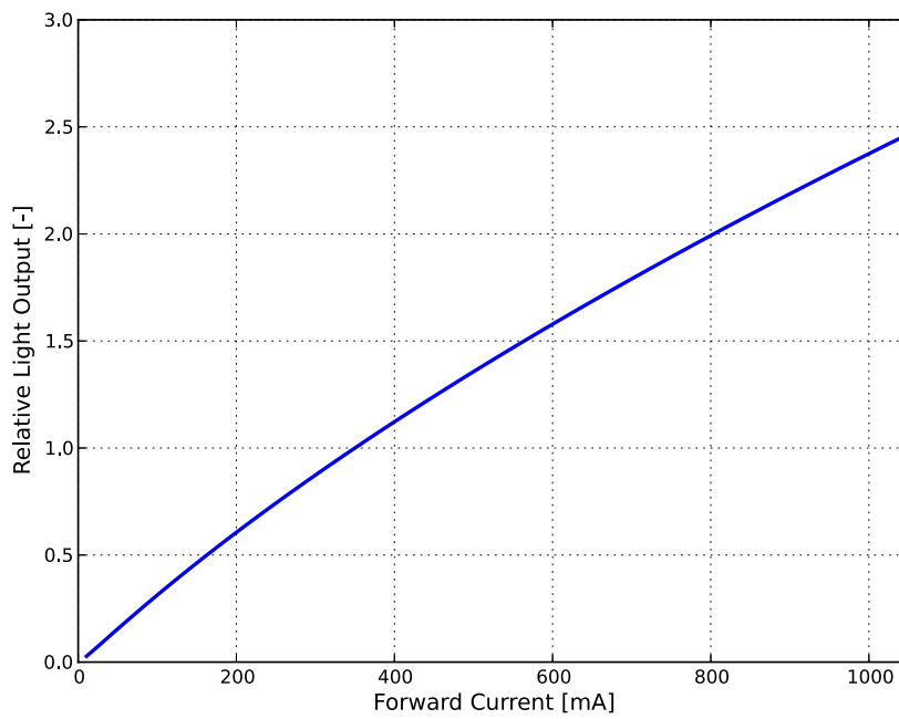
Figure 7. Typical relative luminous flux vs. forward current, LIQ0-xyy00000zzz0.
