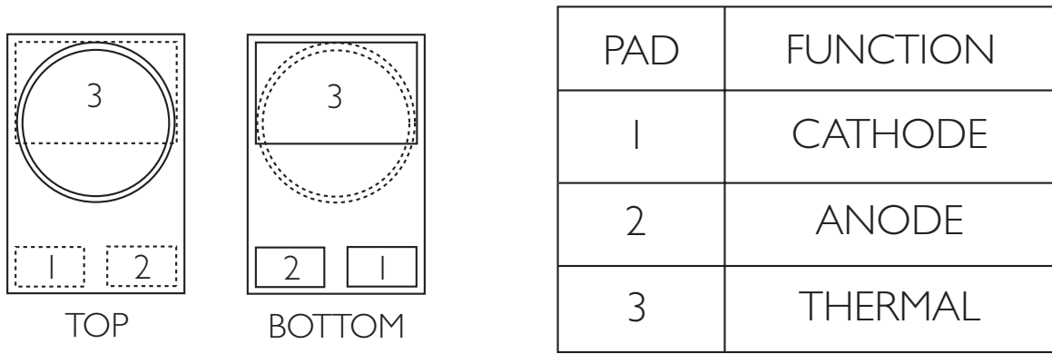
Figure 2. Pad configuration.
