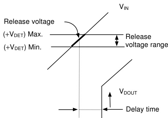
Figure 30 Release Voltage
