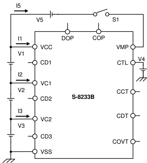
Test circuit 3
