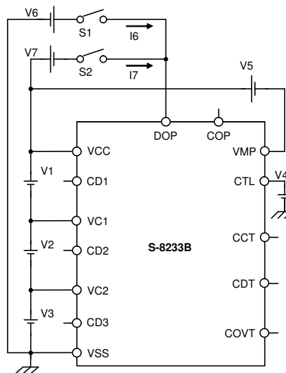
Test circuit 4
