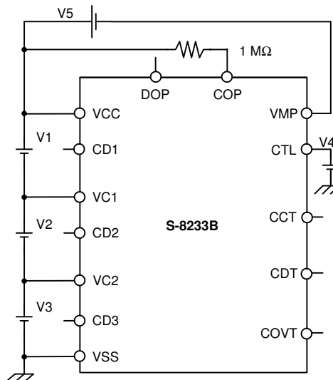
Test circuit 2
