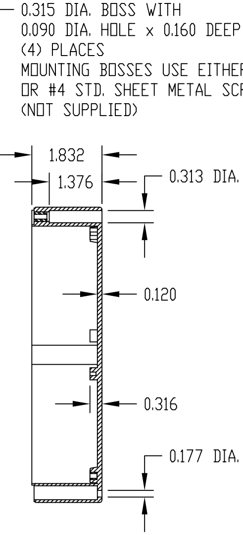
SECTION "A-A"
