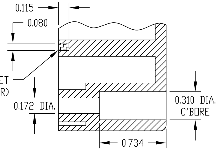
DETAIL "D"
