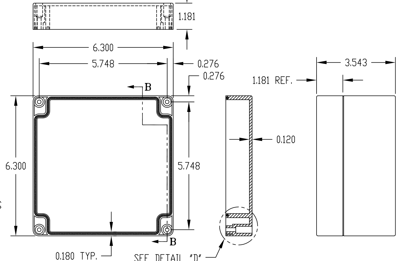
SECTION "B-B"
