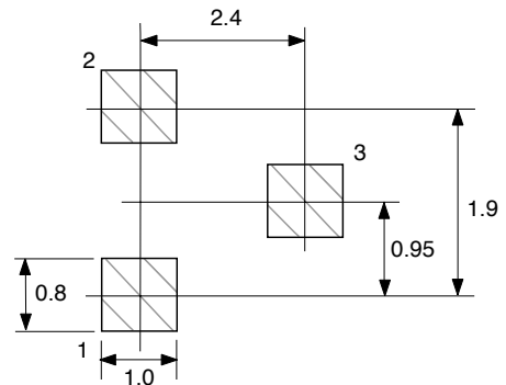
OUTLINE 33 RECOMMENDED P.C.B. LAYOUT
