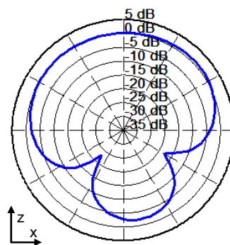
Phi = 0° Plane
