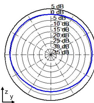
Phi = 90° Plane
