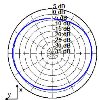
Theta = 90° Plane
