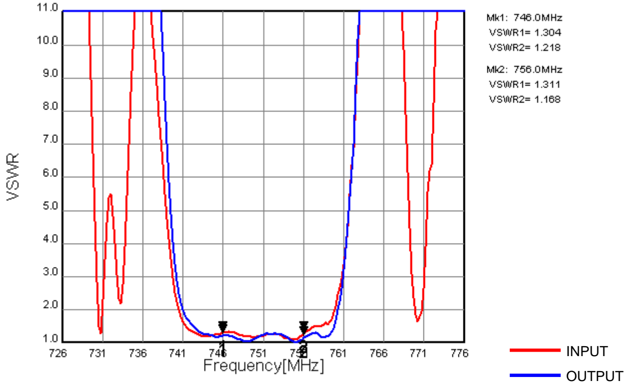
Fig.3 VSWR
