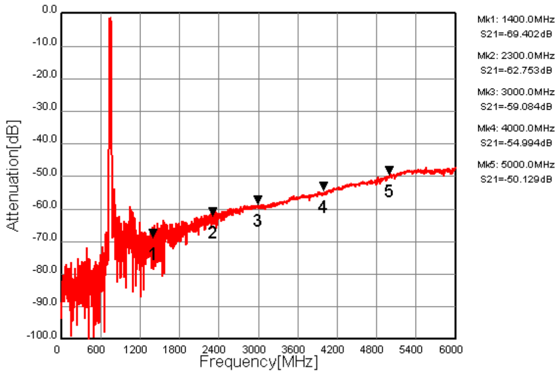
Fig.4 Wide-band Characteristic
