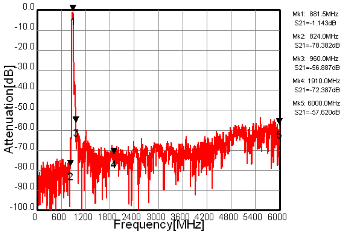
Fig.4 Wide-band Characteristics
